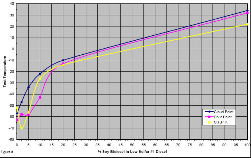
Cold Temperature Properties of Biodiesel Blends
